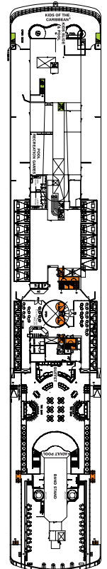
TOP DECK DECK 9
